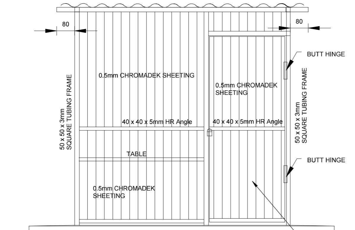
FRONT ELEVATION
