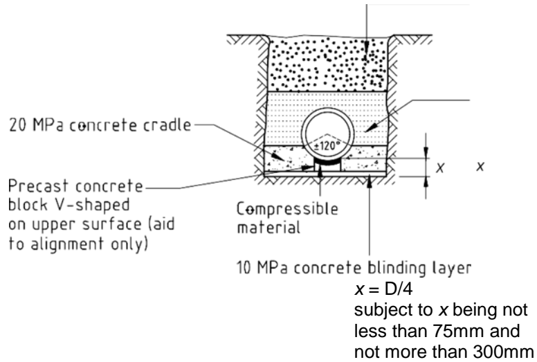
Figure 5 (a): Class A bedding
