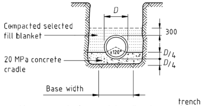
Fig 2 (a) Rigid pipe on Class A bedding
